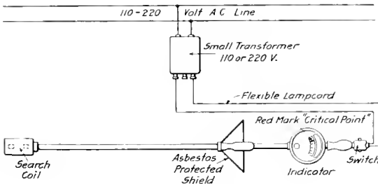
Diagram of Wiring and Pyrometer
